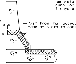
PART SECTION THRU JOINT SEAL
