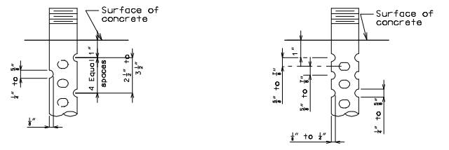
DETAIL OF 3/4" Ø THRU 2 1/2" Ø ANCHOR RODS OPTIONAL DETAIL OF 1 3/8" Ø THRU 2 1/2" Ø ANCHOR RODS
