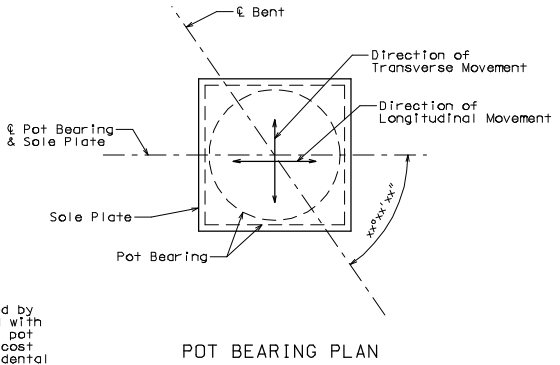
POT BEARING PLAN
