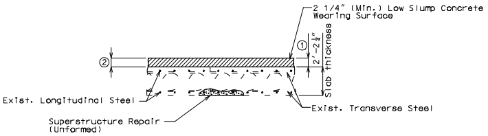
SUPERSTRUCTURE REPAIR (UNFORMED)
