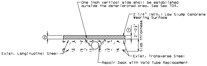
DECK REPAIR WITH VOID TUBE REPLACEMENT
