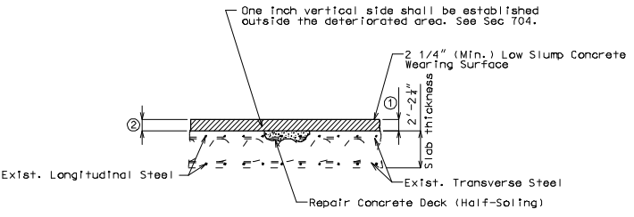
REPAIRING CONCRETE DECK (HALF-SOLING)
