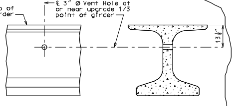
HALF ELEVATION OF GIRDER SPAN (-) Exterior and interior girders are the same, except for coil ties, and coil inserts for slab drains.
