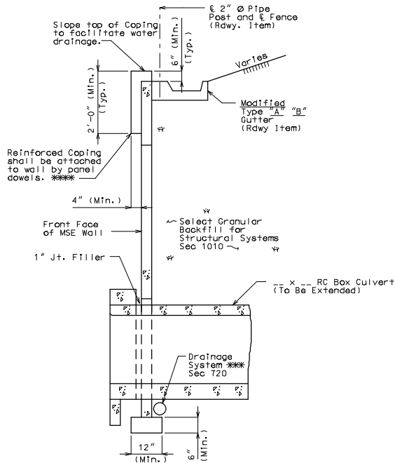
TYPICAL SECTION THRU WALL @ CULVERT
