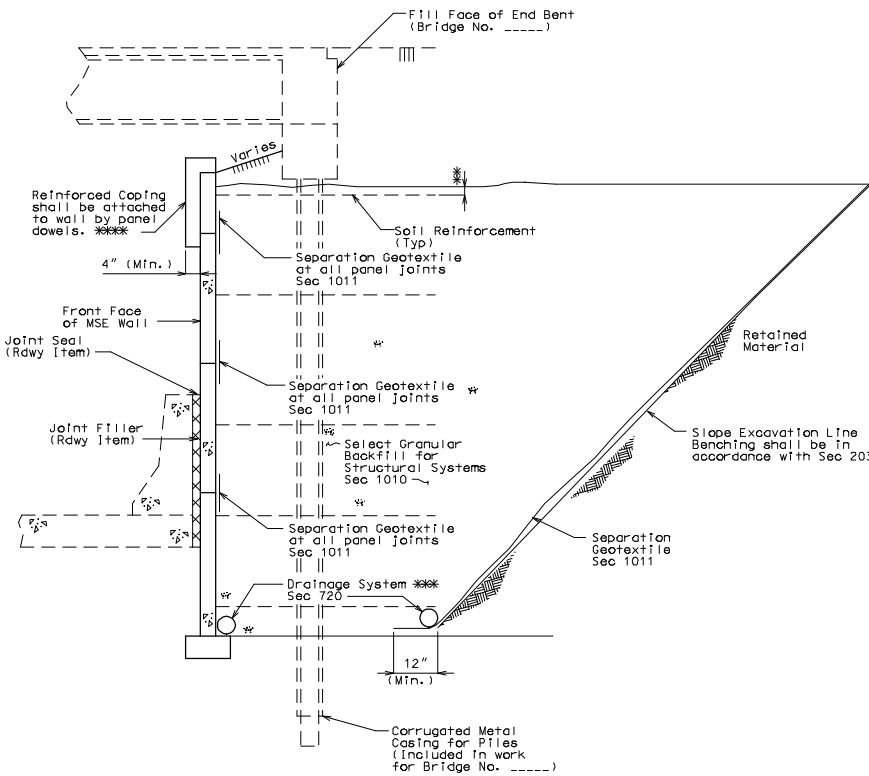
TYPICAL SECTION THRU WALL UNDER BRIDGE
