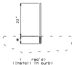
DETAIL OF VERTICAL RESIN ANCHOR SYSTEM
