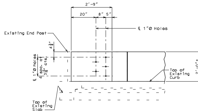
PART SECTION NEAR ENDPST SHOWING HOLE SPACING (REINFORCEMENT NOT SHOWN FOR CLARITY)
