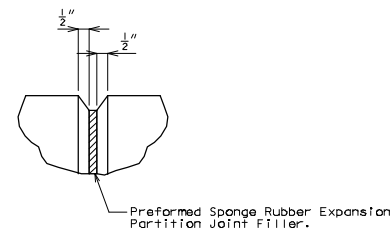
FILLED JOINT DETAIL
