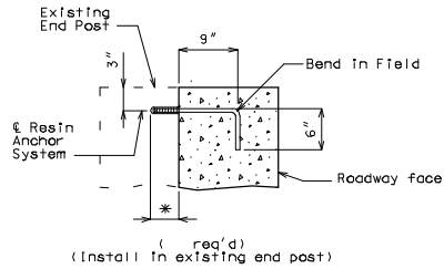
DETAIL OF HORIZONTAL RESIN ANCHOR SYSTEM
