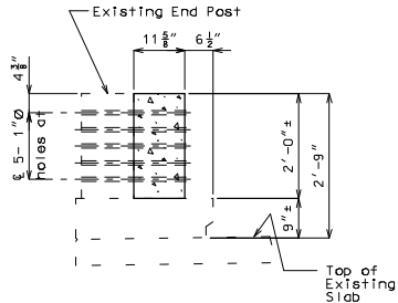
PART SECTION THRU ENDPST SHOWING HOLE SPACING (REINFORCEMENT NOT SHOWN FOR CLARITY)
